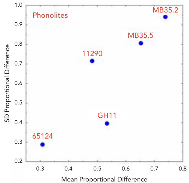
Fig. 8 The difference from the Chatham Islands floater of the five phonolites with the closest chemical composition.
